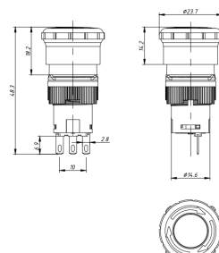
10C emergency stop
