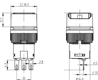
12C square push
