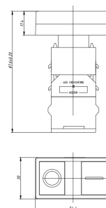
E illuminated double
